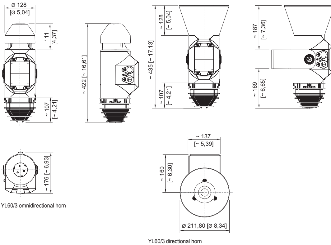
YL60/3 directional horn
